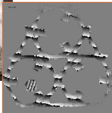
Figure 4b. Dynamic ESPI interferometry measurement data for the structure (Courtesy NASA/Goddard).
