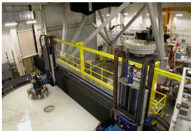
Figure 2. Dynamic interferometry data guides polishing of 8.4 meter and 6.4 meter mirrors (Courtesy Steward Observatory Mirror Lab).
