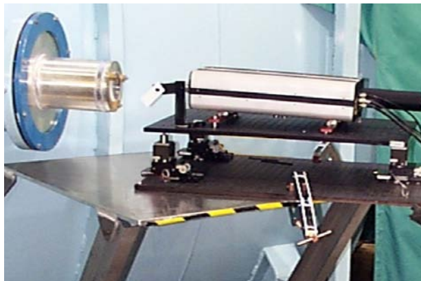
Figure 3. A dynamic interferometer measures a test sample in a vacuum chamber through a view port (Courtesy Ball Aerospace).
