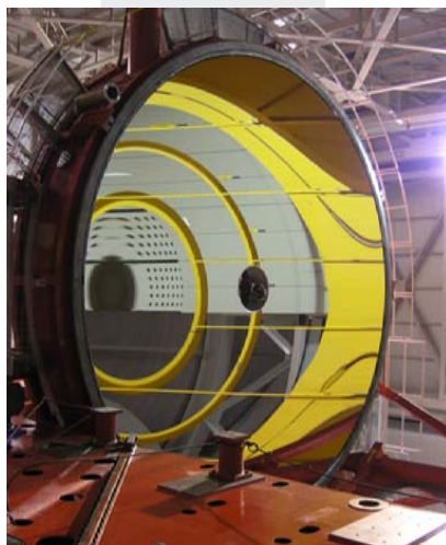
Figure 1. Measurement of large optics, such as this 8 meter primary mirror for the Large Binocular Telescope Observatory, requires metrology systems that can function despite vibration, turbulence and other challenges. (Courtesy R. Bertram and LBTO).
